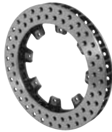
Ultralite 32 Vane 160-5863 11.75" Dia. 160-5865 12.19" Dia. 0.81" Width
