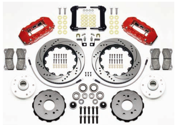
Front Complete Brake Kit
