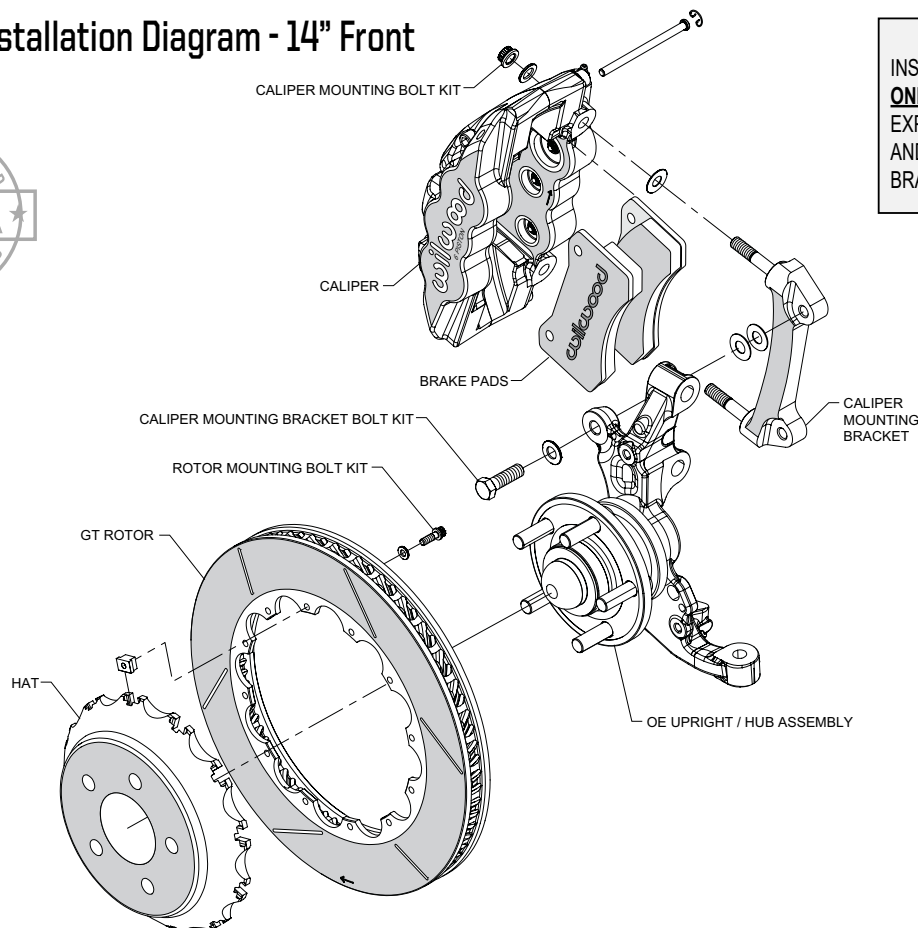
AERO6/ST Front, Spec37 GT Slotted Rotor
