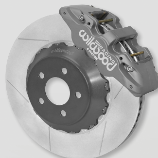
AERO6/ST Front, Spec37 GT Slotted Rotor
