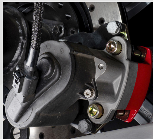
EPB Caliper Mounted
