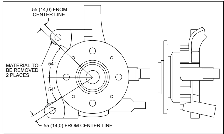
Figure 3. Spindle Modifications
