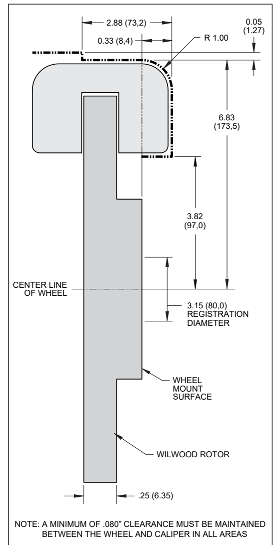
Figure 2. Wheel Clearance Diagram
