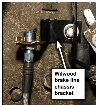
Photo 7b p/n 220-11412 (Bracket mounting)
