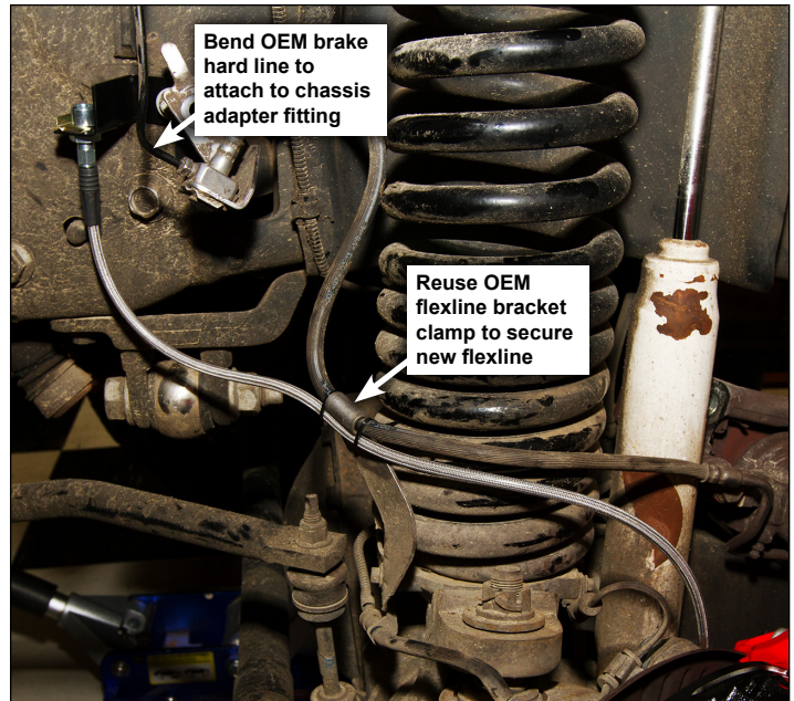
Photo 7a p/n 220-11412 (Flexline shown mocked up)
