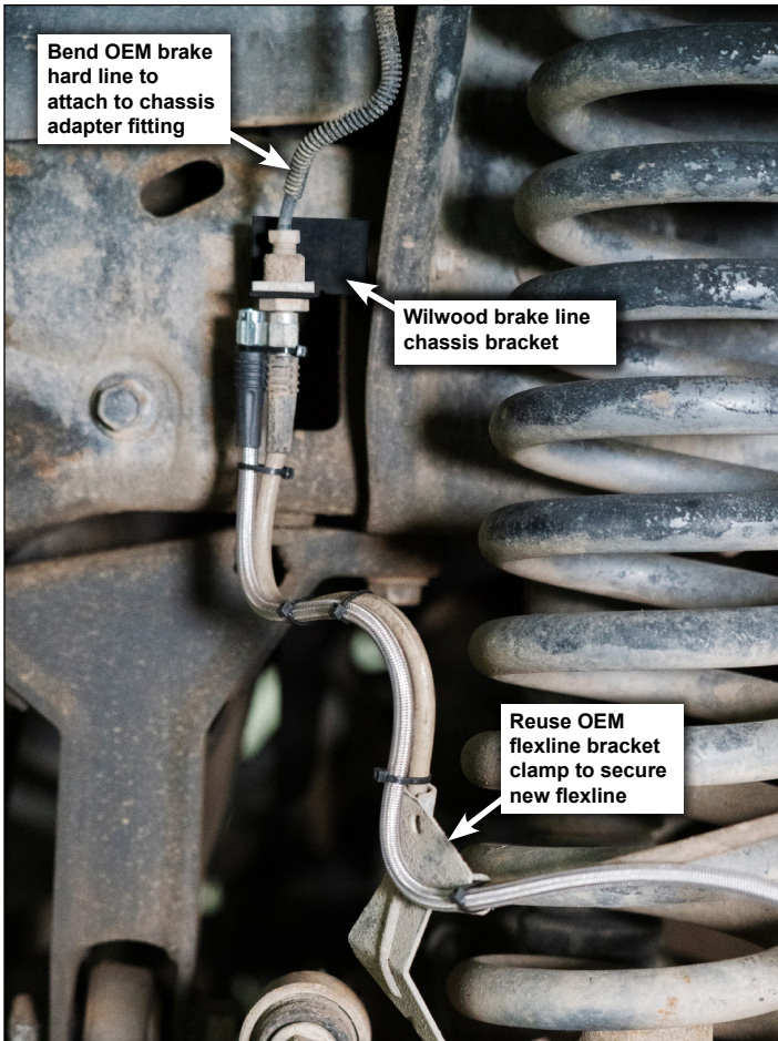
Photo 6 p/n 220-11411 (Flexline shown mocked up)
