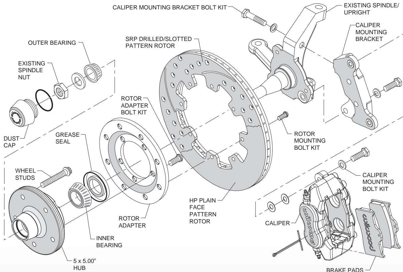
Figure 1. Typical Installation Diagram, Dynalite Kit Shown
