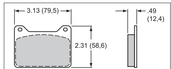
Powerlite Caliper, Type 7912 Pad Dimensions
