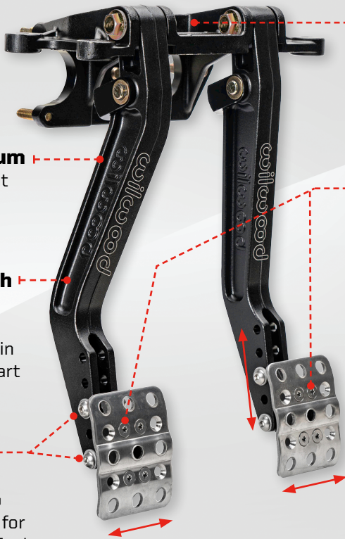
P/N: 340-16833 Brake with Offset Clutch
