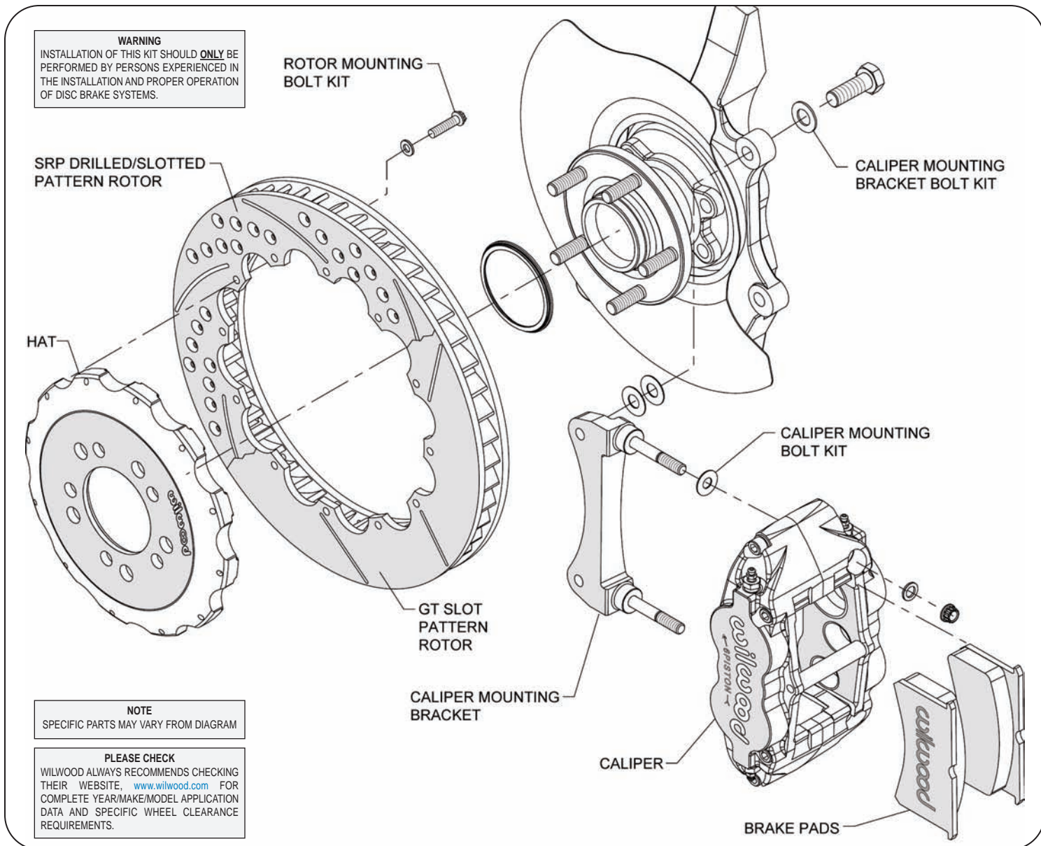
Typical Installation Diagram (13.06" Kit Shown)
