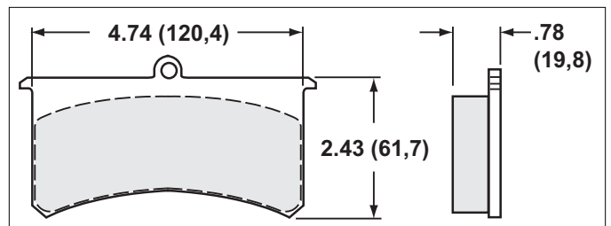
P/N 150-8285K • Superlite with Cotter Pin
