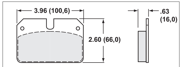
P/N 150-7504K • Narrow Dynalite with Bridge Bolt
