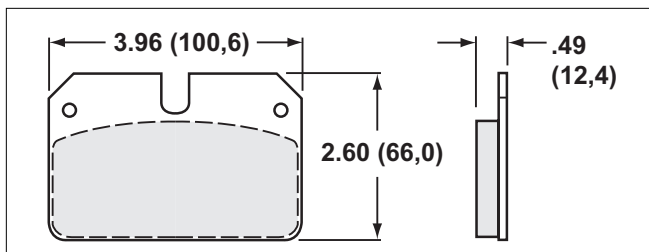
P/N 150-8451K • Dynalite with Bridge Bolt
