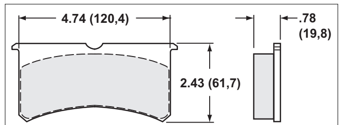
P/N 150-8323K • Superlite with Bridge Bolt
