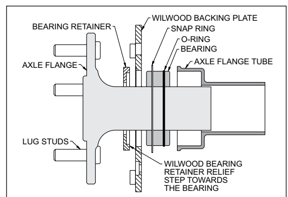
Figure 6. Retainer / Axle Diagram
