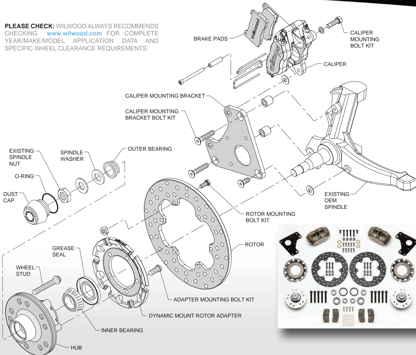
Figure 1. Typical Installation Diagram, 1980-1987 GM "G" Body Shown
