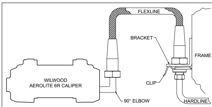
Figure 3. Brake Line Diagram
