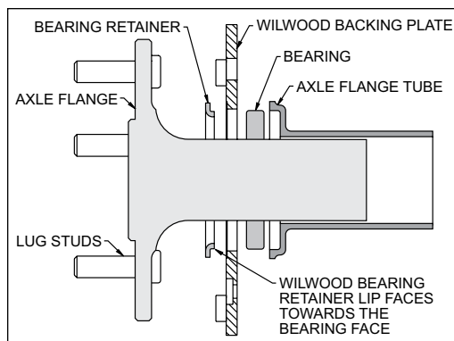
Figure 4. Retainer / Axle Diagram
