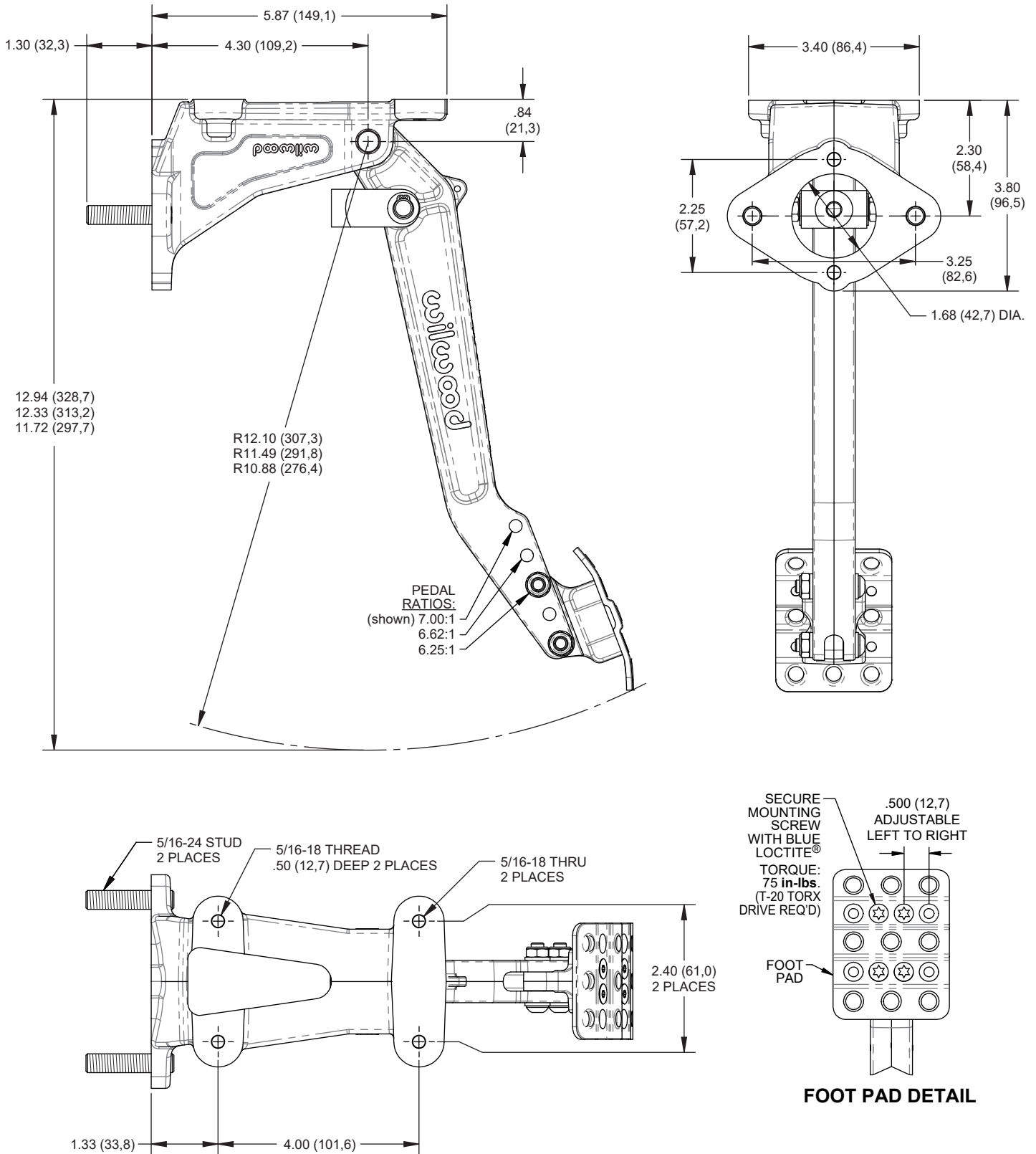
Figure 2. Forward Swing Mount Pedal Assembly, Physical Dimensions, 6.25:1 to 7.00:1 Ratio (p/n 340-17699)
