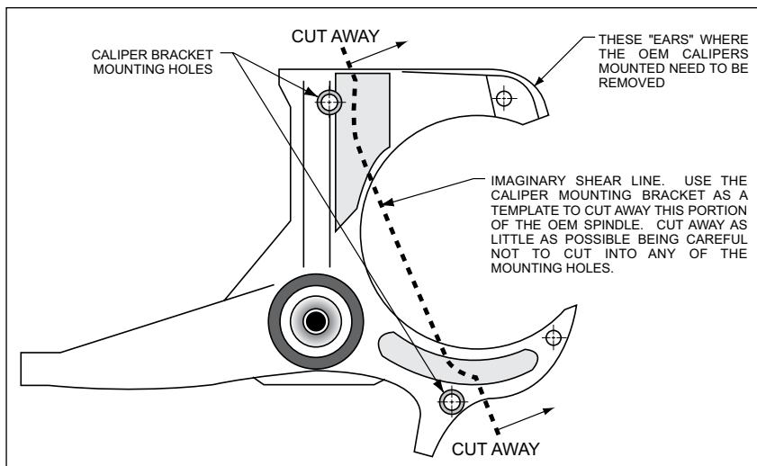
Figure 1. Spindle Modifications
