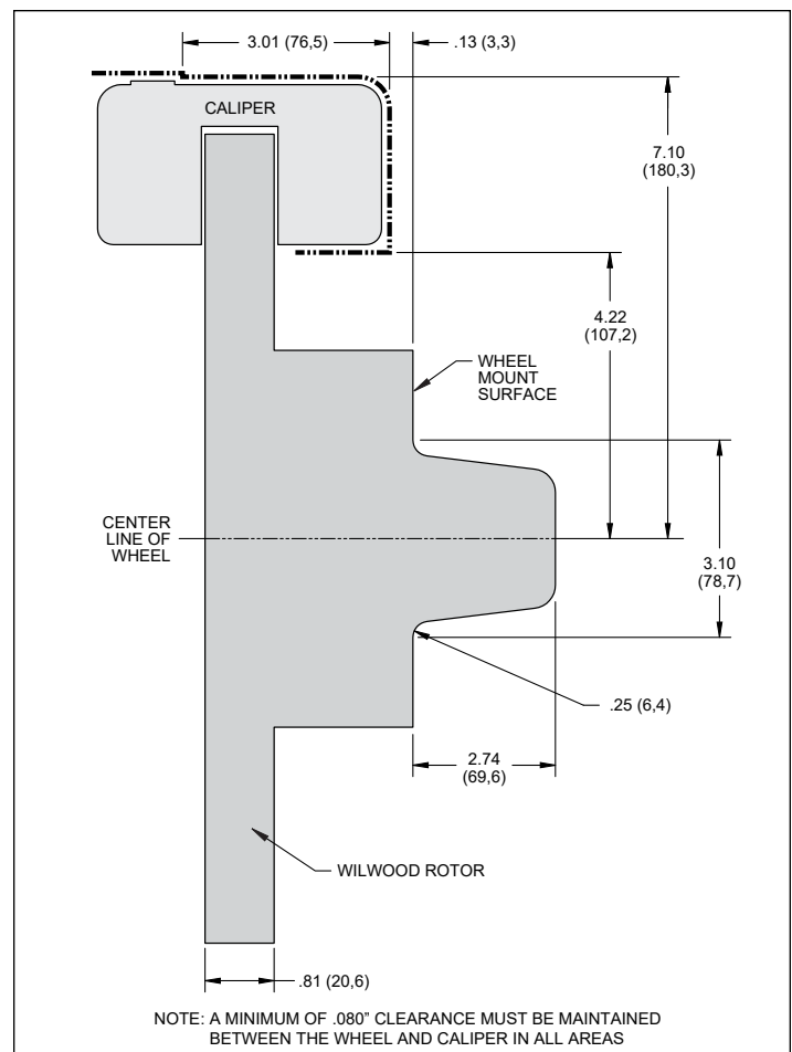
Figure 2. Wheel Clearance Diagram
