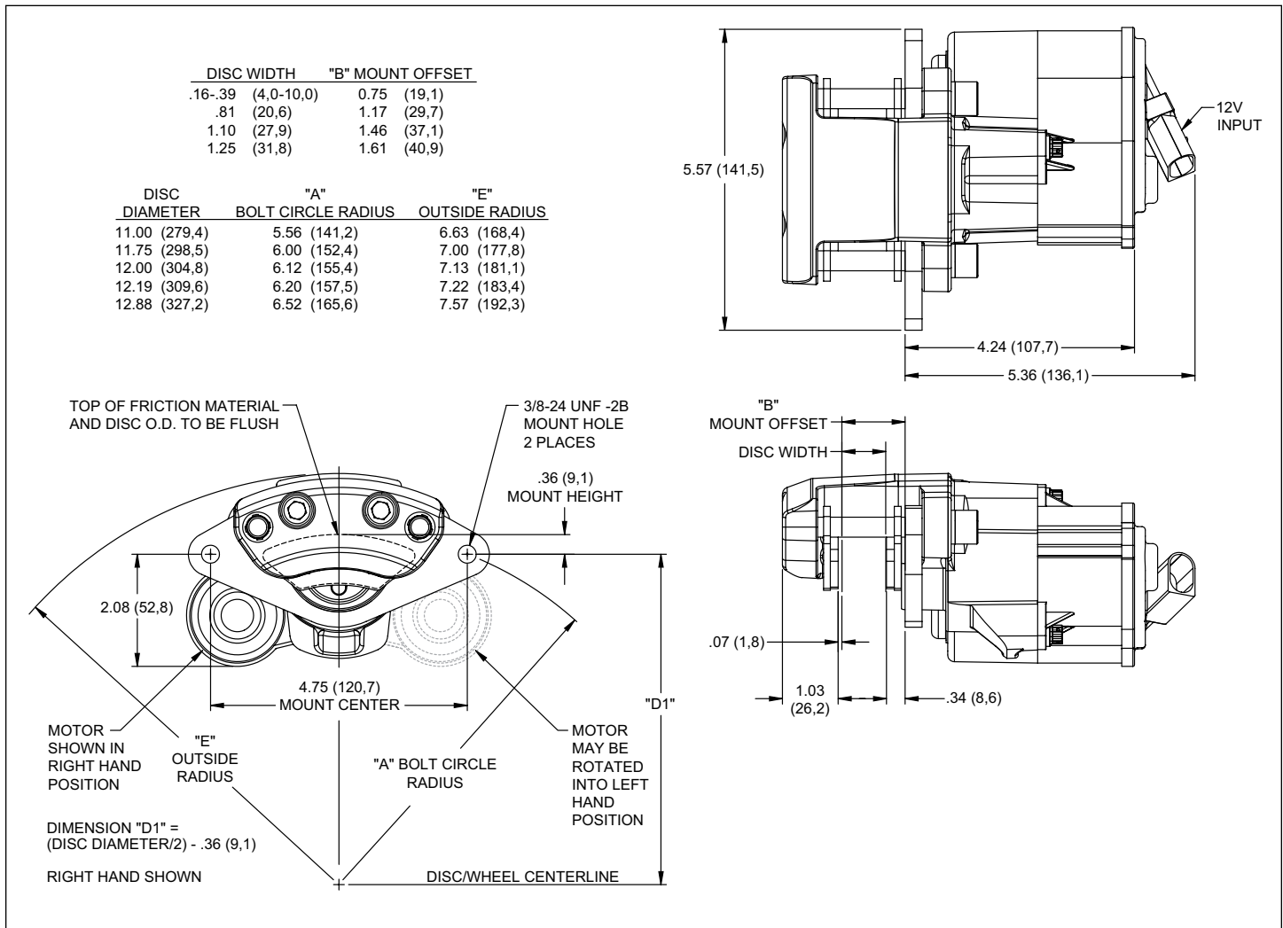
Figure 3. EPB Caliper
